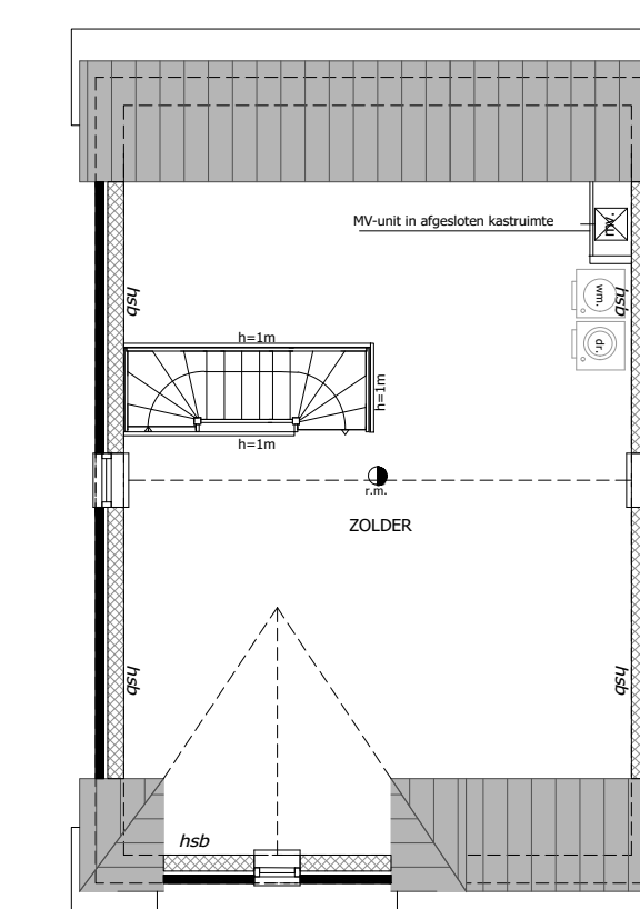
ZOLDER
