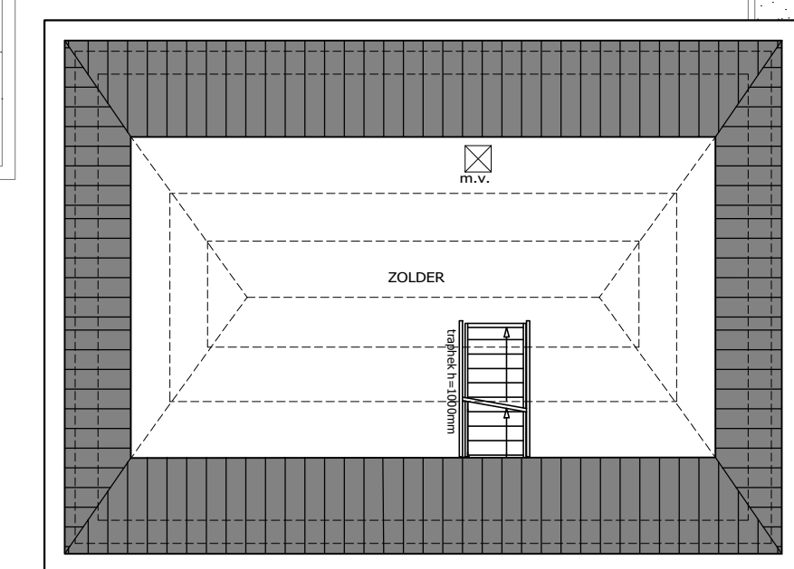
ZOLDER
